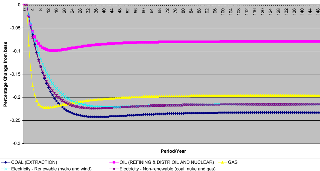
Figure A2.14- Percentage Change in Capital Stocks in the Energy Sectors due to a 5% Improvement in the Aggregate Manufacturing Sector
