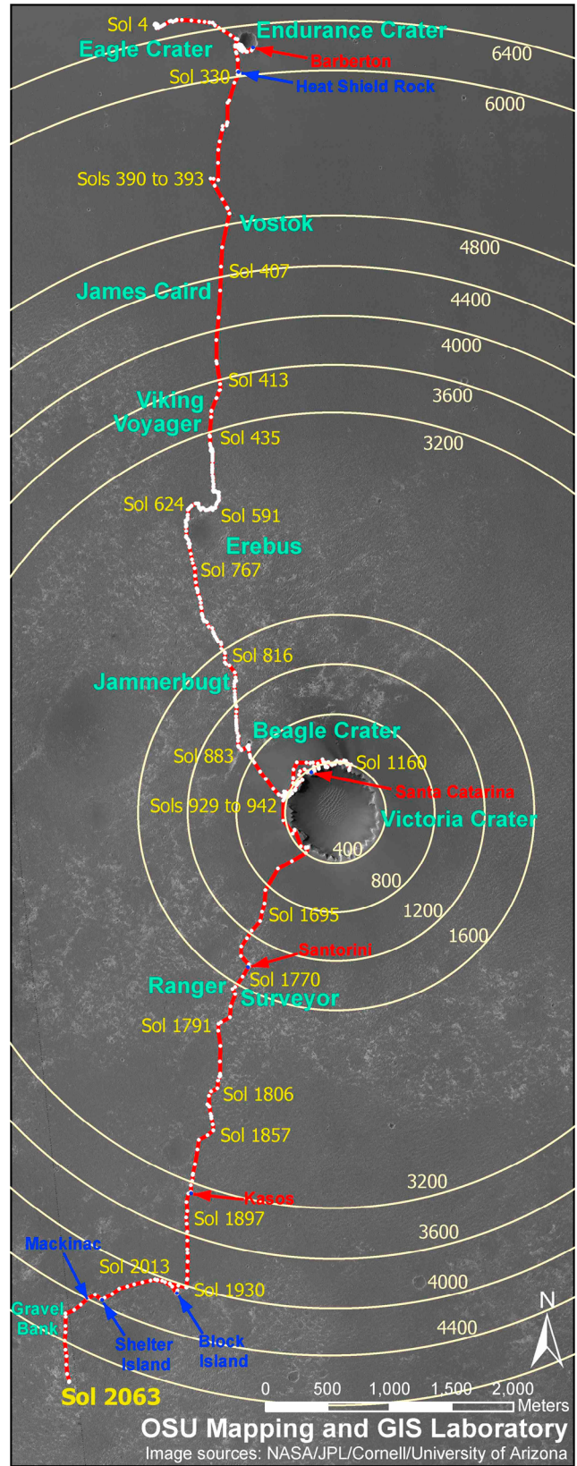
Figure 11. Meteorite finds in relation to Victoria crater. Victoria crater has a diameter of ~800 m (radius of ~400 m). Radii of concentric circles increase in 400 m increments. The map is based on rover positioning data (Li et al., submitted manuscript, 2010).
