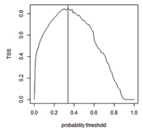
Figure 18. Plot of the True Skill Statistic against probability threshold identifying p=0.35 as the probability threshold for a maximum TSS of 0.86
