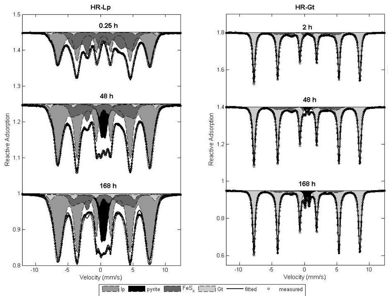
Fig. 5 Mössbauer spectra taken during two HR runs (run 28 and 10). The model parameters used for spectra fitting are listed in Table 2.
