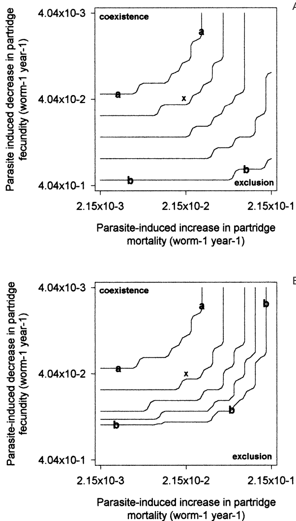
Fig. 6. Exclusion – coexistence boundary curves in the parasite-induced increase in partridge mortality/parasite-induced decrease in partridge fecundity cross-section of parameter space for the pheasant/partridge/ H. gallinarum model detailed by Tompkins et al. (2000 b ) illustrating how the boundary shifts as (A) the parasite-induced decrease in pheasant fecundity is increased logarithmically from its estimated value of 8.28 \times 10^{-4} /worm/year (curve a) to 8.28 \times 10^{-3} /worm/year (curve b), and (B) the parasite-induced increase in pheasant mortality is increased linearly from 0.00 (curve a) to 3.00 \times 10^{-3} /worm/year (curve b). The parameters on both axes are scaled from 0.1 to 10 times their empirical values. Crosses indicate the predicted outcome at the empirical values. The outcome shifts from partridge exclusion to host coexistence when either the decrease in pheasant fecundity is increased to 1.65 \times 10^{-3} /worm/year, or the increase in pheasant mortality is increased to 5.33 \times 10^{-4} /worm/year.
