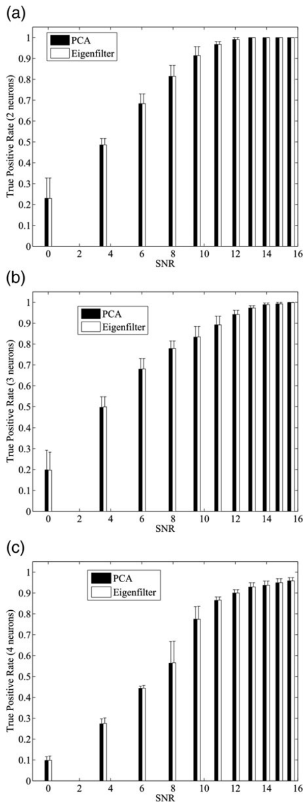
Figure 7 Evaluation of spike sorting accuracy with varied SNR. Comparisons between PCA (Matlab princomp) and stream-based Hebbian eigenfilter are based on (a) 2 neurons (b) 3 neurons (c) 4 neurons cases.
