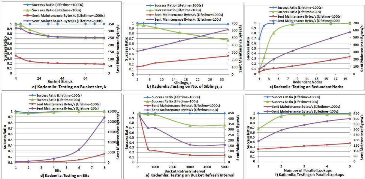
Fig. 6. Kademia: Selecting best parameters according to a) Bucket size, b) No. of siblings, c) No. of redundant nodes, d) Bits per digits, e) Bucket refresh interval and f) No. of parallel lookups.
