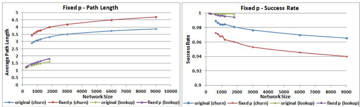
Fig. 3. Average path length and success rate with fixed p .
