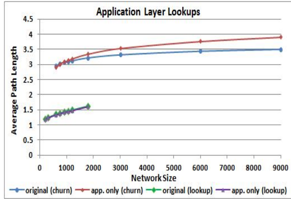
Fig. 2. Comparison of average path length with APPLICATION lookups only vs. all lookup.
