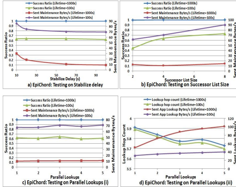
Fig. 8. EpiChord: Selecting best parameters according to Stabilize delay, b) Successor list size, c) Parallel lookups(i) and d) Parallel lookups (ii).
