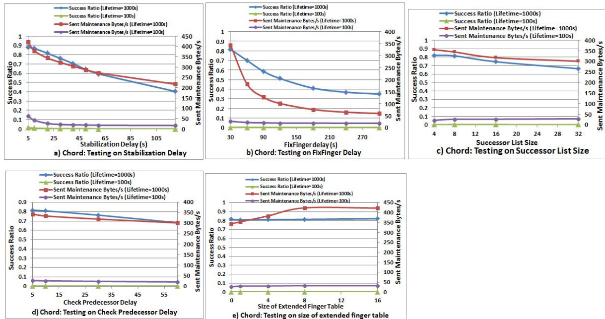
Fig. 4. Chord: Selecting best parameters according to a) stabilization delay, b) fixfinger delays, c) successor list sizes, d) check predecessor delays and e) extended finger table sizes.
