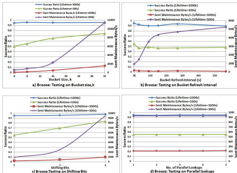
Fig. 7. Broose: Selecting best parameters according to a) Bucket size, b) Bucket refresh interval, c) Shifting bits and d) No. of Parallel lookups.
