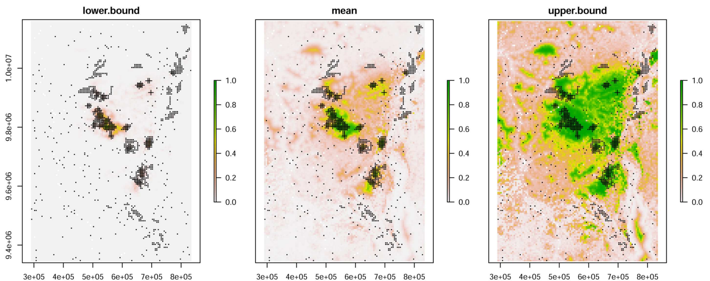
Fig 2. The mean (centre) and 95% confidence interval (left: lower bound; right: upper bound) of the probability of presence for Grauer's gorilla. The maps also show the location of cells sampled (grey dots) with cells where gorilla sign was observed (black crosses).
