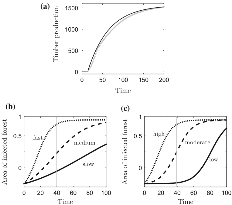
Fig. 1 Timber production and disease progress curves. In a the data points (grey dots) are the timber production ( \text{m}^3 \text{ha}^{-1} ) from the forest yield model for unthinned, yield class 14 Picea sitchensis against time (years). The fitted curve (black) is produced using Eq. (11) and the parameters are in Table 1. The area of infected forest ( L - x(t) ha) is plotted against time (years) with b a fixed rate of primary infection and three secondary infection rates and c a fixed rate of secondary infection and three primary infection rates (the parameter sets are in Table 2). The optimal rotation length of the disease-free system, T_{DF} , is shown as a vertical, grey line
