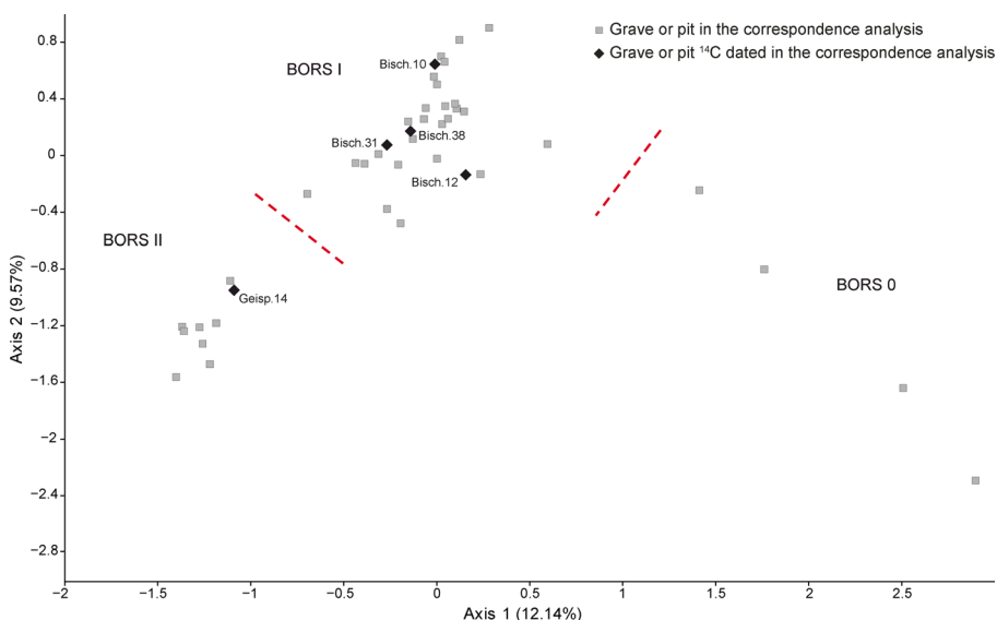
Fig. 13 Correspondence analysis of BORS pottery in Lower Alsace
