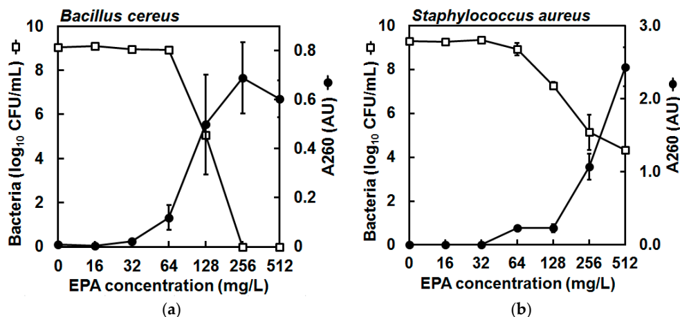
Figure 3. Enumeration of colonies from cell suspensions of (a) Bacillus cereus NCIMB 9373 and (b) Staphylococcus aureus Newman in PBS ( \square ) and detection of 260-nm (A260)-absorbing material in cell-free filtrates ( \bullet ) after exposure to increasing concentrations of eicosapentaenoic acid (EPA) during 30 min at 37 °C, showing that the number of viable cells in suspension reduced concomitant to the amount of A260-absorbing material in cell-free filtrates, indicating likely cell membrane perturbation and cell lysis. The bacterial inoculums at the start of incubation were 1.51 \times 10^9 \pm 0.41 \times 10^9 CFU/mL (mean \pm standard error) and 1.57 \times 10^9 \pm 0.15 \times 10^9 CFU/mL for B. cereus and S. aureus , respectively. The carrier solvent (ethanol) had little effect on bacterial viability and at the greatest concentration of ethanol (2.56%, v/v) the bacteria recovered at 30 min was 1.31 \times 10^9 \pm 0.10 \times 10^9 CFU/mL and 2.79 \times 10^9 \pm 0.05 \times 10^9 for B. cereus and S. aureus , respectively (data not shown). Meanwhile, control incubations in the presence of carrier solvent (ethanol) showed that negligible quantities of A260-absorbing material were detected in cell-free filtrates (data not shown). Data are mean (geometric mean for CFU values) \pm standard error (not all error bars are visible); n = 3 for A260 values, n = 2 for CFU/mL determinations (detection limit was 2 \log_{10} CFU/mL); note that the secondary y-axis (A260) scales differ for (a,b).
