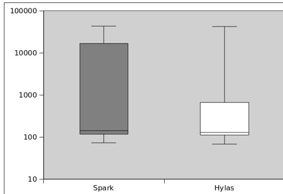
Fig. 2. Boxplot for Spark vs HYLAS execution times given in seconds
