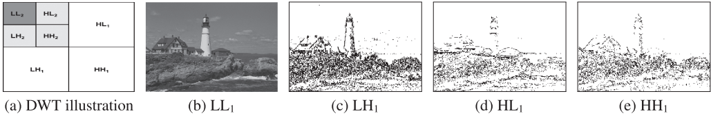
Fig. 9. Example of multiresolution wavelet decomposition, where (b), (c), (d), and (e) are level 1 approximation ( LL_1 ), vertical ( LH_1 ), horizontal ( HL_1 ), and diagonal ( HH_1 ) subbands, respectively.
