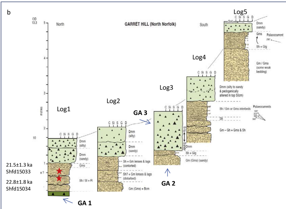
Fig. 16. a) Location of Garret Hill, North Norfolk. The MIS 2 ice limit is marked running west to east (Straw, 1960). b) Sediments sections from the northwest side of the Garret Hill showing gravelly diamict separated by stratified sand and gravels. OSL dates from the lower sands provide ages of 21.5 \pm 1.3 and 22.8 \pm 1.8 ka (Shfd15033 and Shfd15034; Table 1).
