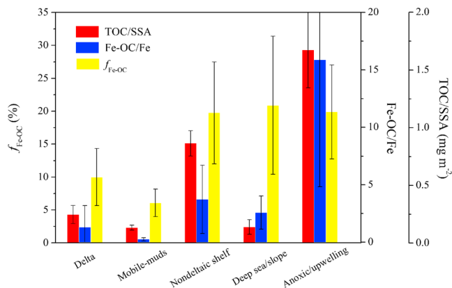
Figure 6. The TOC/SSA loadings, Fe-OC/Fe ratios, and f_{Fe-OC} in different marine environments. The TOC/SSA ratios are from Aller (1998) and Yao et al. (2014). The Fe-OC/Fe ratios and f_{Fe-OC} are from Lalonde et al. (2012), Ma et al. (2018), Salvadó et al. (2015), Shields et al. (2016), and this study. Deltaic regions included the Changjiang delta (including mobile muds and shelf), Makenzie river delta, and the Wax Lake Delta (Lalonde et al., 2012; Shields et al., 2016; and this study). Mobile muds included the ECS mobile muds (this study); nondeltaic shelf regions included the Mexican Margin, Madeira turbidite, Arabian Sea, Eurasian Arctic Shelf, middle and outer shelf of ECS, and South Yellow Sea (Lalonde et al., 2012; Ma et al., 2018; Salvadó et al., 2015). Deep Sea/slope regions included the Southern Ocean, Equatorial Pacific, and Station M (Lalonde et al., 2012). Anoxic/upwelling regions included the Black Sea, Mexican Margin, Indian Margin, Lake Brock, and Saanich Intlet (Lalonde et al., 2012). TOC = total organic carbon; SSA = specific surface area.
