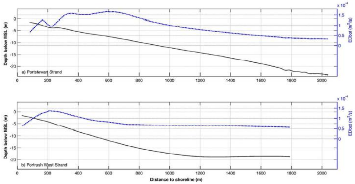
Figure 7. Energy dissipation due to bottom-friction (dashed blue line) along the nearshore profile (solid grey line) of Portstewart Strand (a) and Portrush West Strand (b). Modelled ED_{bot} values for the peak storm conditions at 00:00 of June 22 nd .
