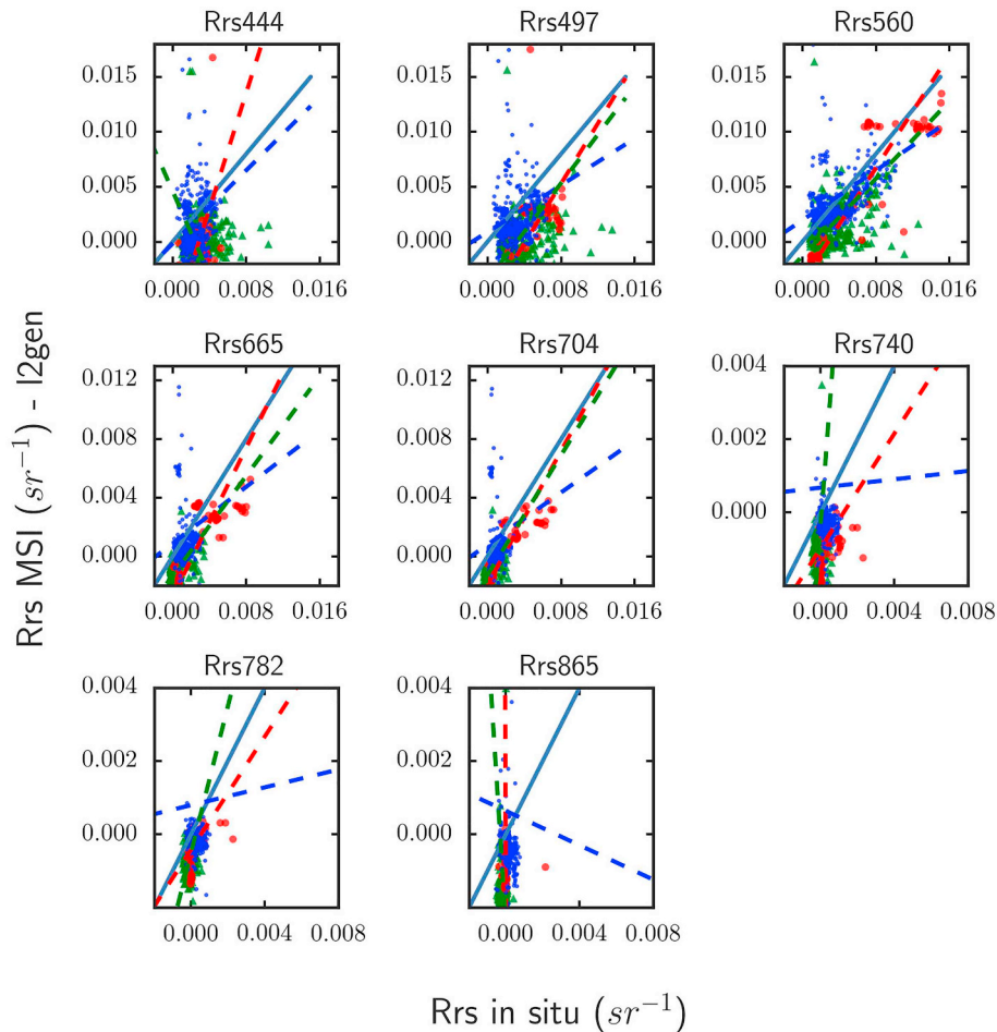
Fig. 7. I2gen per-band scatter plots. Colours and symbols are as in Fig. 4. (For interpretation of the references to colour in this figure legend, the reader is referred to the web version of this article.)
