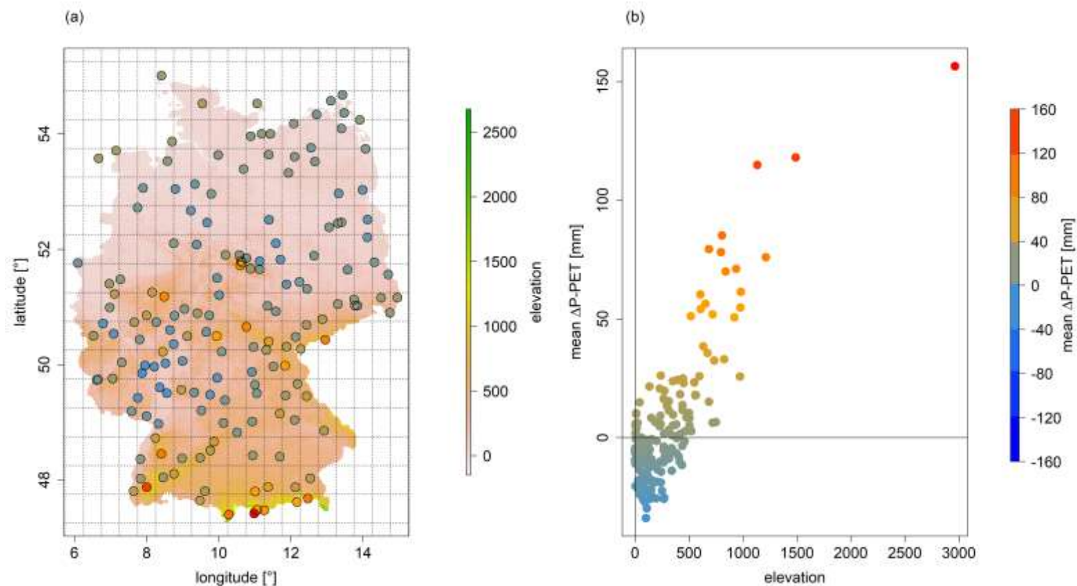
Figure S5. Mean differences of P-PET ( \text{mean } \Delta P\text{-PET} ) estimates as derived from DWD (German meteorological service) climate station data as well as gridded climate products (CRU TS v 3.24.01). The map (a) depicts the location of climate stations (colored dots with color scale referring to the legend in (b)) on top of a digital terrain model (background colors with color scale referring to the legend in (a)). Dashed lines demarcate the nodes of the CRU 0.5^\circ grid. The scatterplot (b) reflects the dependence of mean \Delta P\text{-PET} on elevation. Coloration of the dots corresponds to the same colors as in (a). Positive values indicate that P-PET as derived from gridded climate data underestimates the climate station based estimate. Thus, overestimation of P-PET (blue dots, negative values) largely occurs at low elevations while underestimation (orange and red dots, positive values) mostly occurs at high elevations.
