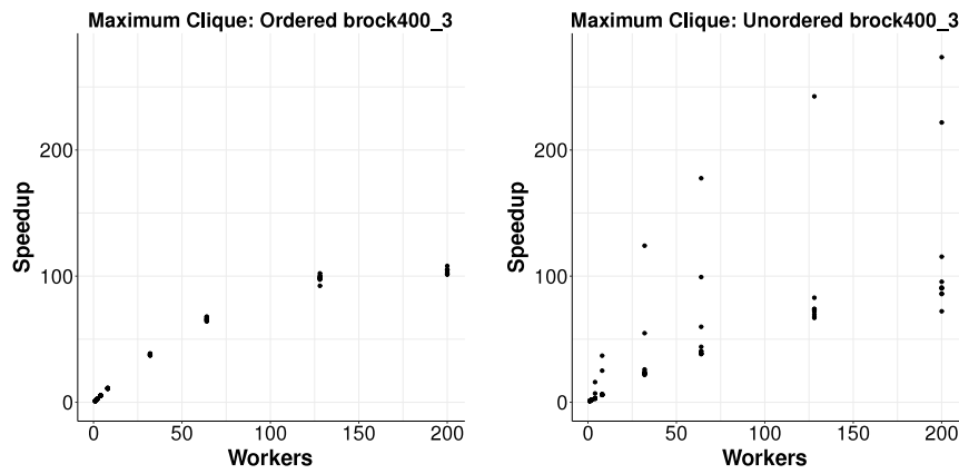
Fig. 7. Unordered skeleton violates Non-increasing Runtimes: Sampled speedups for maximum Clique.
