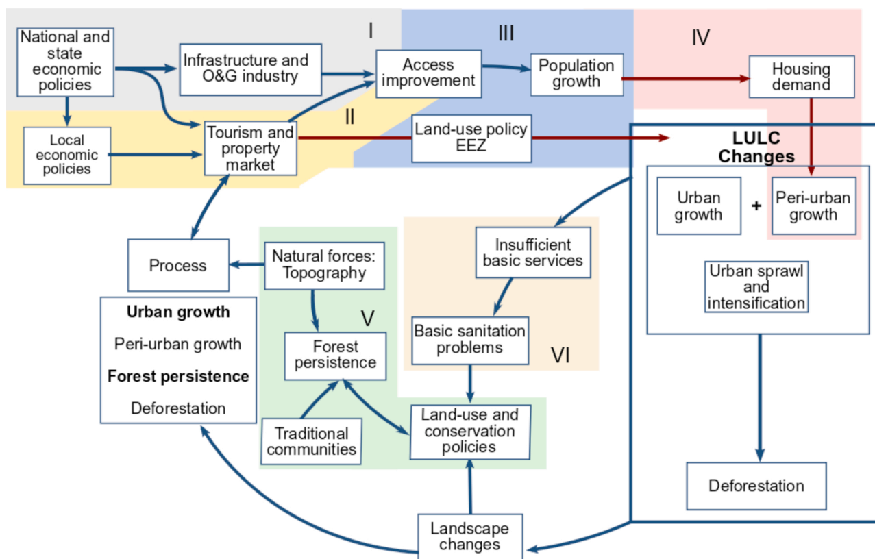
Fig. 9. Conceptual interlinkages between drivers of processes in NCSF from 1985 to 2015. (I) national and state economic policies, responsible for increasing investment in oil and gas (O&G) industries and for expanding access by roads and seaports (end of 20th century); (II) local and regional economic policies, governed mainly by tourism and the real estate and construction market (end of 20th and early 21st century); (III) items I and II were responsible for labour migration (end of 20th century) and have influenced the regional land-use policies (early 21st century); (IV) the resident population has been excluded from access to the housing market, and this has led to the occupation of peripheral peri-urban areas by new housing (end of 20th and early 21st century); (V) conservation policy and traditional communities have been extremely important for forest conservation and for the maintenance of forest cover (end of 20th and early 21st century); (VI) the percentage of public service provision did not follow the urban and peri-urban growth.
