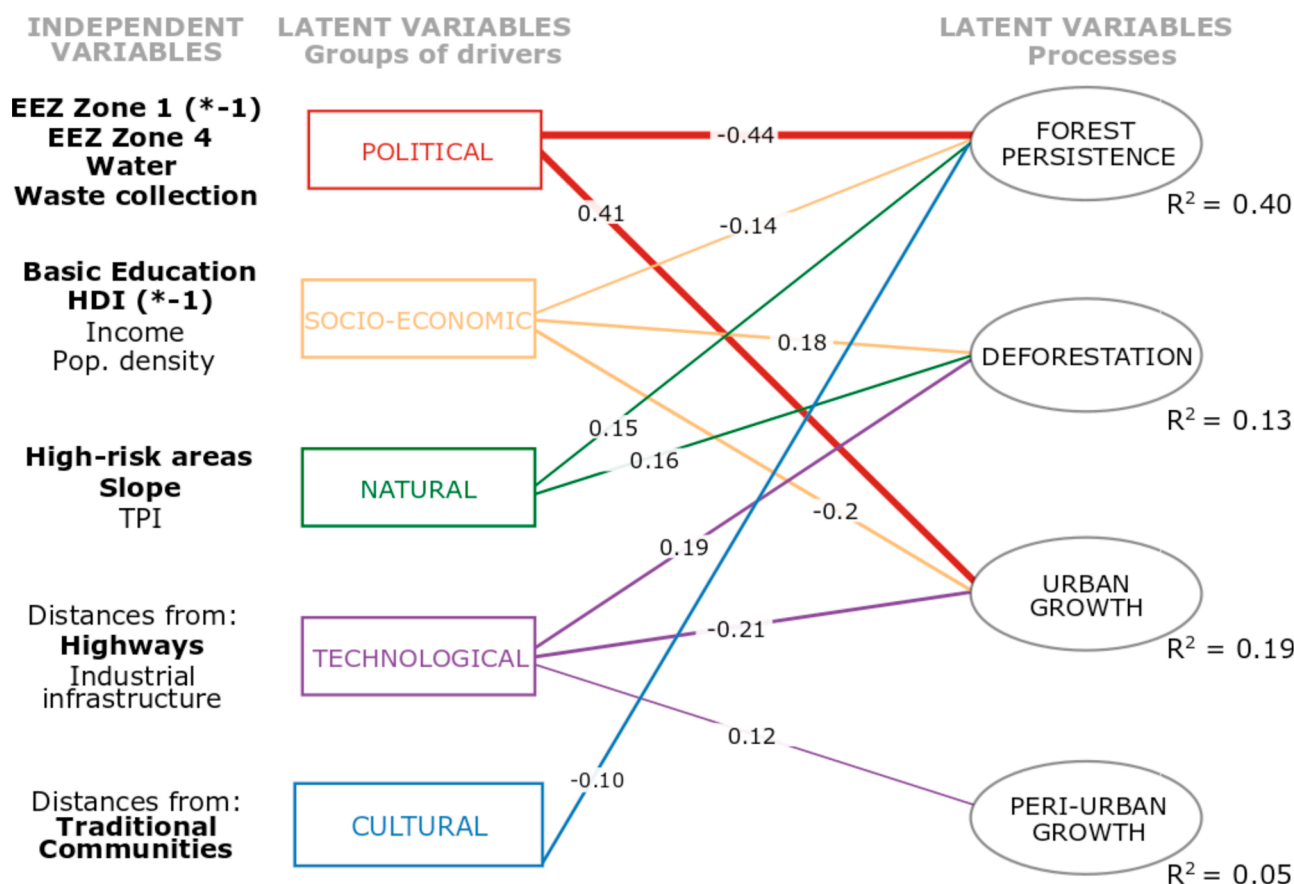
Fig. 8. Model for the study area outside State Park limits for 2000 to 2015. In Bold : Explanatory variables (driving forces) with effect >0.7 and weight >0.5. Coefficient of contribution (C) values with an absolute value >0.1 are displayed.
