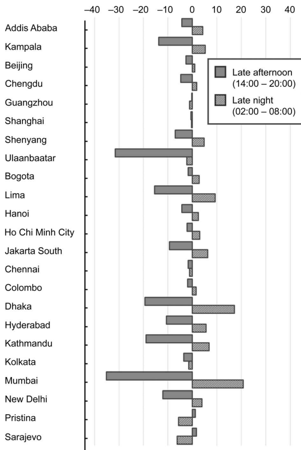
Figure 5 Difference between mean annual outdoor PM_{2.5} concentration in the late afternoon (14:00–20:00) and at night (02:00–08:00) by LMIC city, 2018. PM_{2.5} = particulate matter smaller than 2.5 \mu m in diameter; LMIC = low- and middle-income country.
