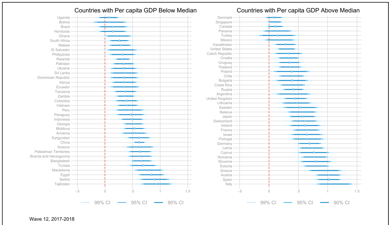
Figure 4. Within-country life satisfaction-income gradient for wave 12 (2017-2018). Note. GDP = gross domestic product.
