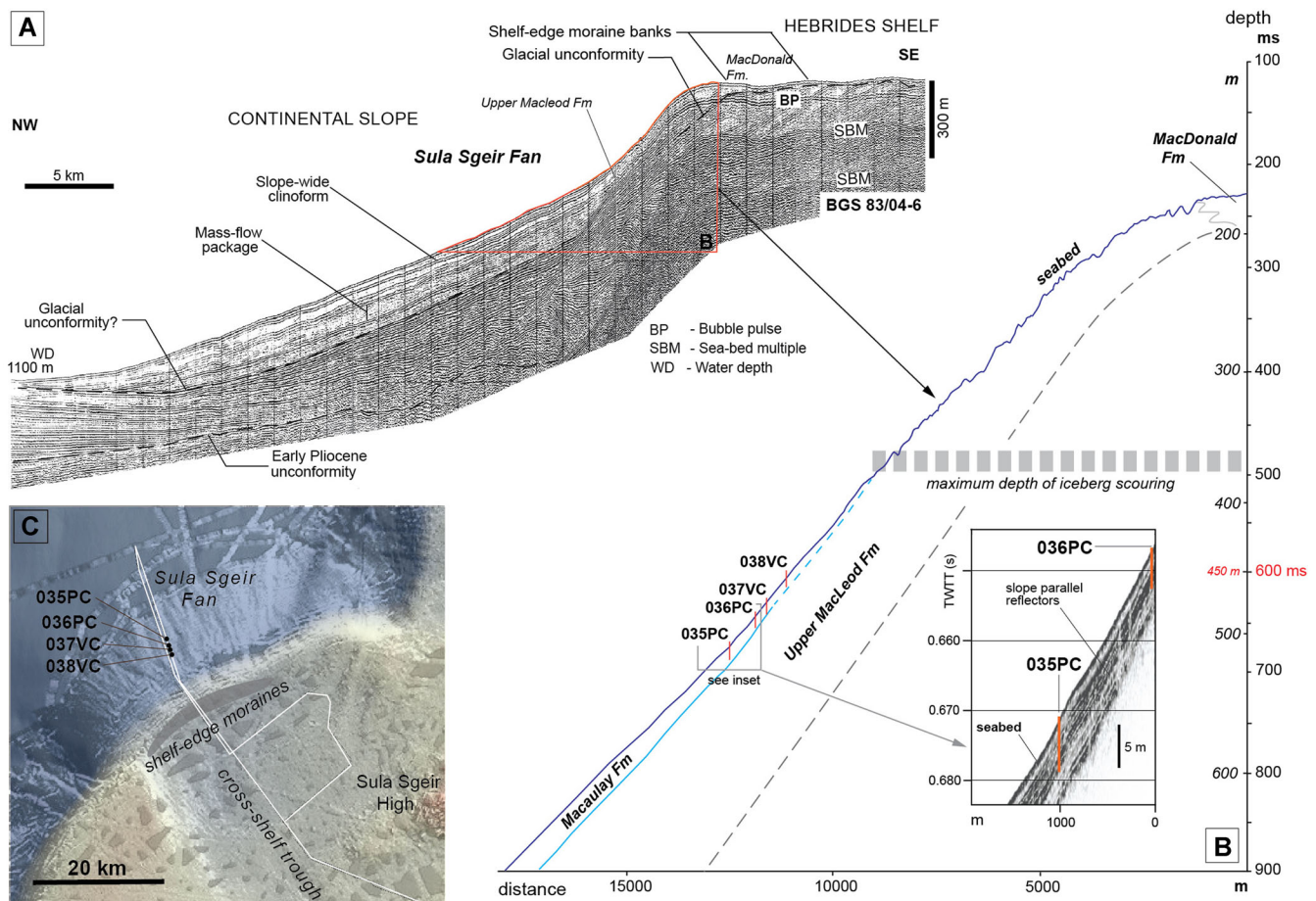
Figure 11. Marine geophysical data from the Sula Sgeir Fan, Continental Slope, offshore NW Scotland. (A) BGS airgun profile across outer Hebrides Shelf and continental slope showing seismic architecture of Sula Sgeir Fan (from Stoker and Bradwell, 2005). Section in panel B highlighted orange. (B) Bathymetric profile of upper Sula Sgeir Fan showing location of cores taken below maximum depth of iceberg scouring on slope. Inset panel shows sub-bottom profile (SBP) data on slope from core sites 035PC and 036PC. TWTT = two-way travel time. A velocity of 1500 \text{ m s}^{-1} was used to convert TWTT into depth. (C) Singlebeam echosounder bathymetry (Olex dataset) highlighting the macroscale geomorphology of the Sula Sgeir Fan at the mouth of the adjacent cross-shelf palaeo-ice-stream trough. White line is data collection track (JC123); core sites on slope are labelled. [Color figure can be viewed at wileyonlinelibrary.com ]
