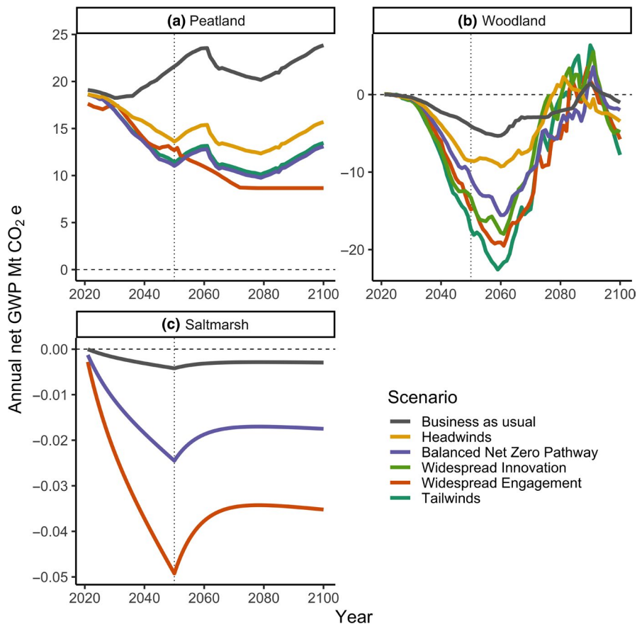
FIGURE 2 Annual GWP_{100} for three NbS options under a range of scenarios. For (a) peatlands, the Widespread Engagement scenario includes restoration of 100% of afforested peatlands. For (c) saltmarsh, sequestration under Headwinds and Widespread Innovation follow Balanced Net Zero Pathway, and Tailwinds follows Widespread Engagement. For context, UK annual emissions in 2018 were 451 Mt CO_2e (BEIS, 2020)
