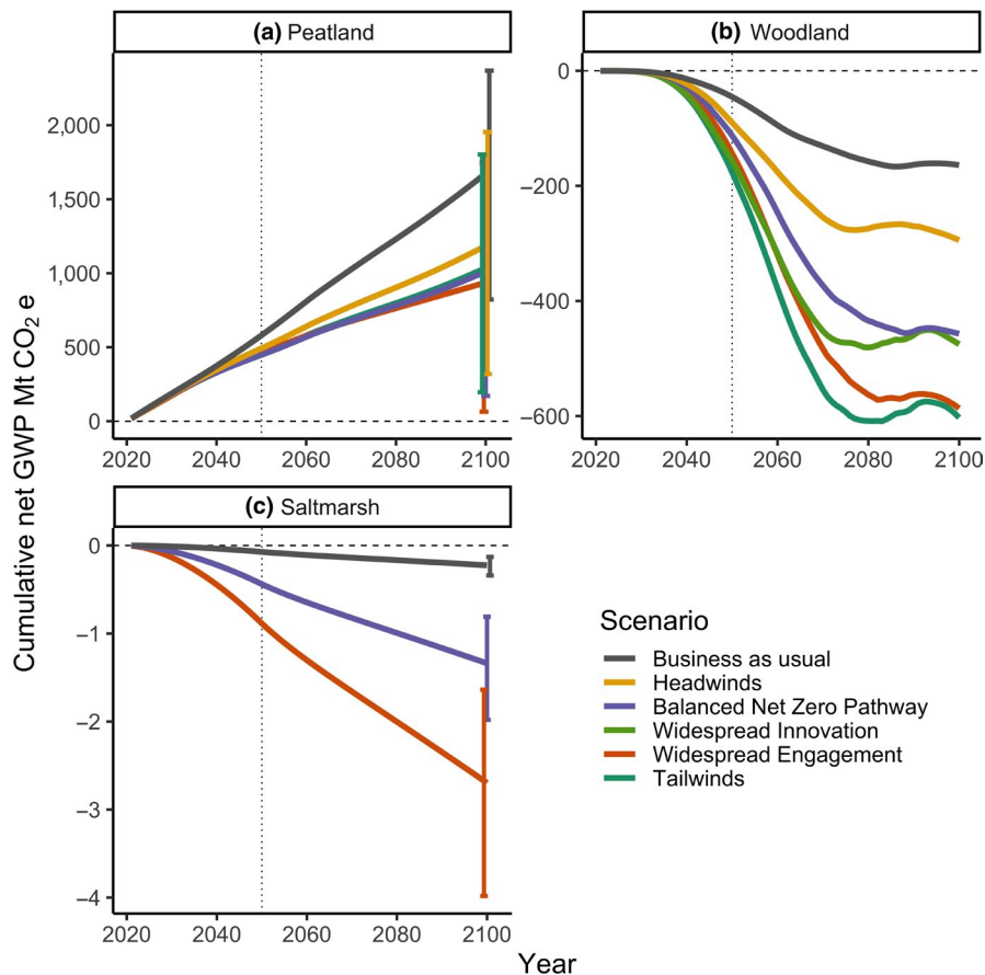
FIGURE 1 Net GWP_{100} for three NbS options under a range of scenarios. Restoration and creation are complete by 2050, shown by the dotted vertical line. For (a) peatlands, 95% confidence intervals are shown by the error bars at 2100, representing cumulative uncertainty. The Widespread Engagement scenario includes restoration of 100% of afforested peatlands. For (b) woodlands, no measures of uncertainty in sequestration are provided by the Woodland Carbon Code. For (c) saltmarshes, error bars show cumulative uncertainty as mean values \pm 1 SD. Sequestration under Headwinds and Widespread Innovation follow Balanced Net Zero Pathway, and Tailwinds follows Widespread Engagement
