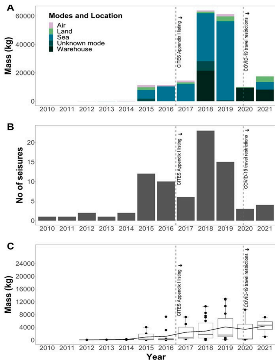
Fig. 2. Yearly reported confiscated mass of seizures linked to Nigeria from January 2010 to September 2021 showing the associated modes of transport or location of pangolin derivatives when confiscated (A). Yearly reported number of confiscations linked to Nigeria from January 2010 to September 2021 (B). The mean mass per seizure linked to Nigeria from January 2010 to September 2021 (line; left y-axis), and a boxplot showing confiscated masses of each seizure event (black dots), median mass (horizontal line in each box), and largest and smallest masses for each year (whiskers) (C). From left to right, vertical dashed lines indicate a) when CITES ban on commercial international trade was brought into effect (January 2017), and; b) when global COVID-19 travel restrictions were made (approximately April 2020). Mass data were not included in panels B and C for 2011 and 2012 (count data were available for these years). Data for 2021 ends in September.
