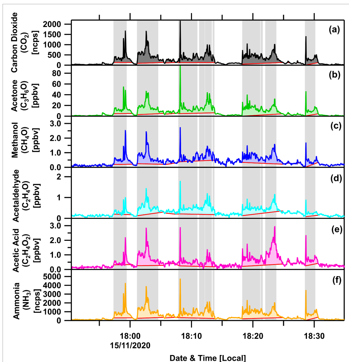
Figure 5. Example time series of CO 2 (a), acetone (b), methanol (c), acetaldehyde (d), acetic acid (e) and ammonia (f) concentrations after a running minima background has been subtracted and the contribution from non-breath sources have been identified and removed by PMF. The solid red line represents an interpolated background between the period before and after the cow enters the BMP. The presence of the cow was determined on the basis of a CO 2 concentration >135 ncps. The coloured shaded areas represent the portion of the signal that would be attributed to the animal within the BMP and the grey shaded areas indicate the periods where an animal visited the breath monitor platform.
