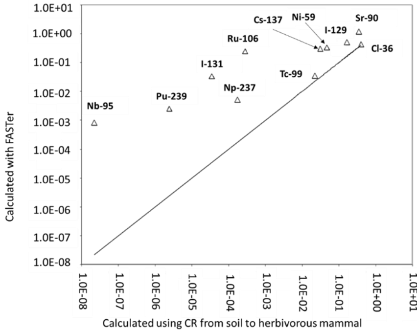
Figure 2. Activity concentrations ( \text{Bq kg}^{-1} \text{ FM} ) in herbivorous mammals 50 years after a continuous constant deposition ( 1 \text{ Bq m}^{-2} \text{ y}^{-1} ) onto a semi-natural ecosystem, calculated with the computer programme FASTer (Avila et al. 2004), which includes a direct external contamination pathway, with root uptake modelled using CR_{wo-soil} (reproduced from Brown et al. 2003).
