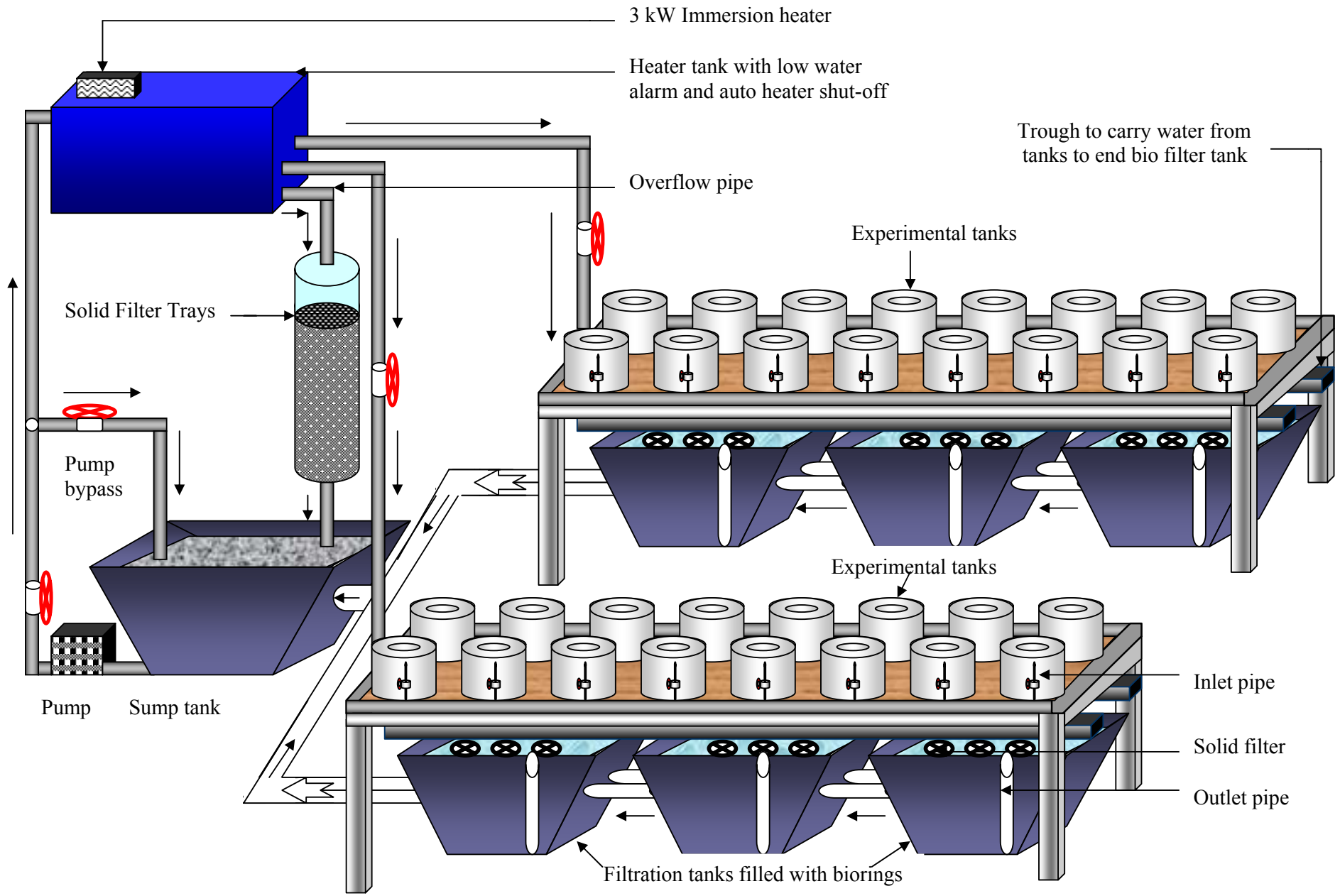
Figure 2.1 Schematic three-dimensional view of experimental system
