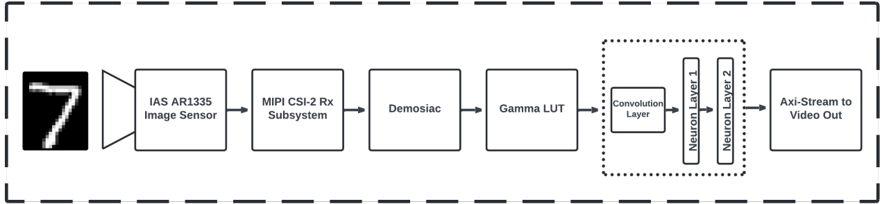
Figure 2. Implementation of Spiking Neural Network on FPGA.
