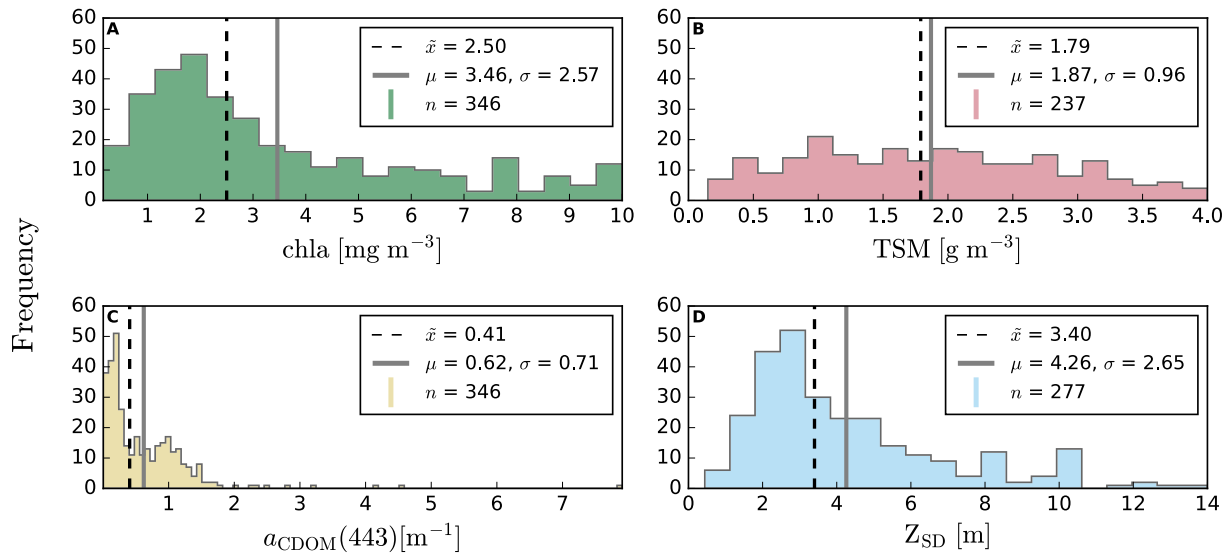
Fig. 4. Parameter distributions of the dataset. (A) chl a , (B) TSM, (C) a_{CDOM}(443) and (D) Z_{SD} . Denoted are the median ( \tilde{x} ), mean ( \mu ) and standard deviation ( \sigma ) of the respective parameter.
