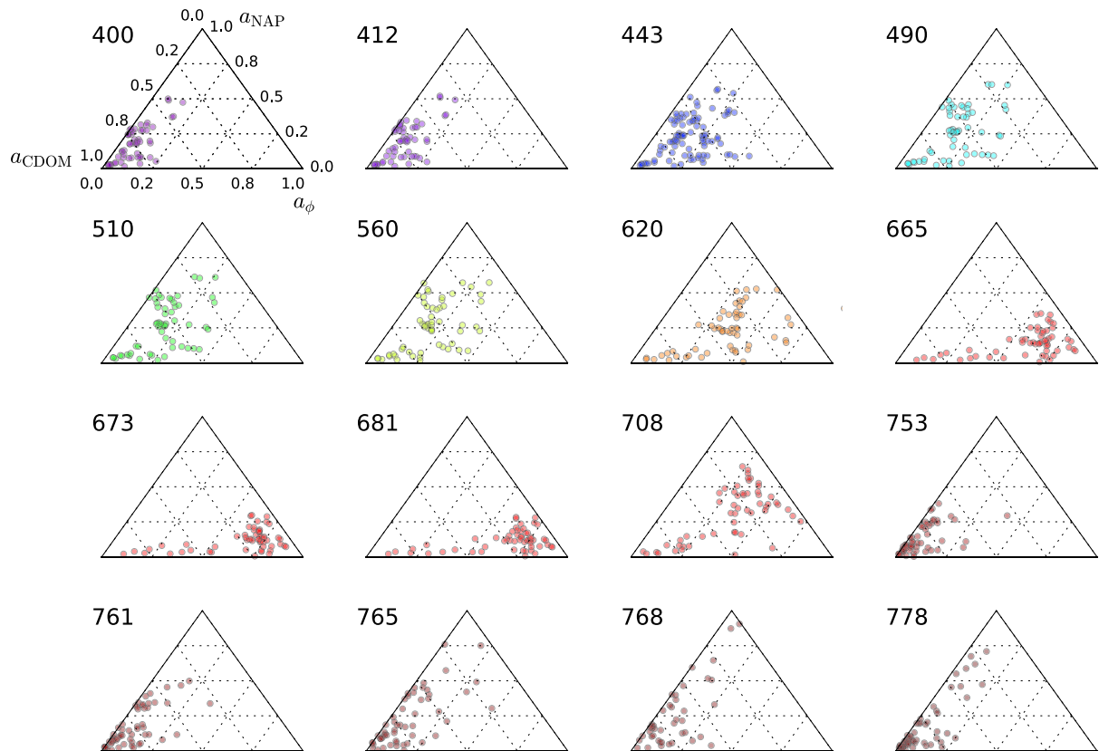
Fig. 5. Ternary diagrams of absorption ( a_{\phi}(\lambda) , a_{NAP}(\lambda) and a_{CDOM}(\lambda) ) for OLCI bands. Measurements where a_{\phi}(\lambda) < 0.01 were excluded.
