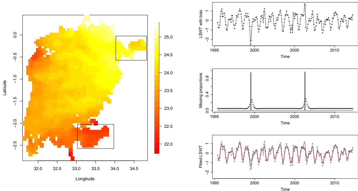
Figure 4: (Left) A map showing the lake surface water temperature data (in °C) from Lake Victoria in July 1999 and the two areas (black boxes) used to create the biased mean LSWT. (Right) The centred LSWT time series from Lake Victoria with inserted biased data shown as red triangles (top), the missing proportion time series and the \alpha_k , k = 1, \dots, K series (middle), and the smoothed LSWT time series from standard P-spline smoothing (blue curve) and adaptive smoothing (red curve) (bottom).
