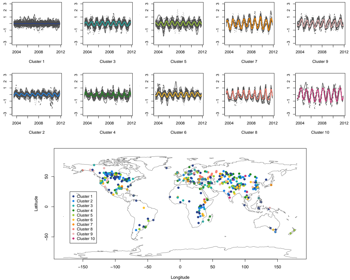
Figure 7: (Top) The smoothed seasonal signals extracted from the centred \log(\text{Chl-}a) from ten clusters (grey curves) and the curves representing the cluster centers (colourful curves). (Bottom) The clustering result shown on a map, where each dot represents a lake and the colour represents the cluster membership.
