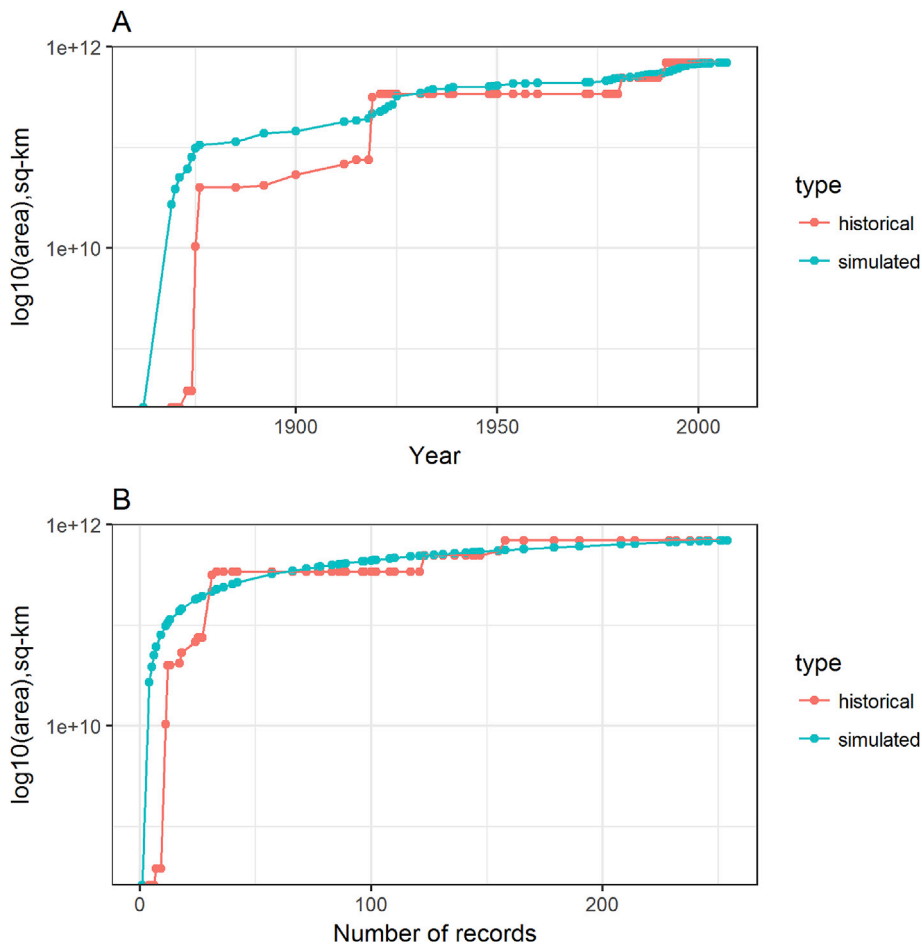
Fig. 1. Geographic range accumulation curves for satyr tragopan ( Tragopan satyra ). A, Comparison of historical (red curves) and simulated area accumulation curves (green curves) for year. B, Comparison of historical and simulated area accumulation curves for number of records. When the area of the range based on historical records exceeds that of the range based on simulated records, it indicates that our knowledge of that species' range is better than random. Plots based on N = 1000 iterations and show mean range areas \pm 1SE . Note: Standard errors estimated at each point are so small that they cannot be represented on the plot. (For interpretation of the references to colour in this figure legend, the reader is referred to the Web version of this article.)
