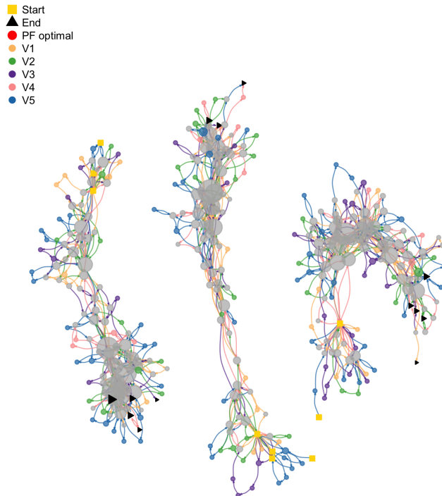
(b) STN of NSGA-II on UF8.
