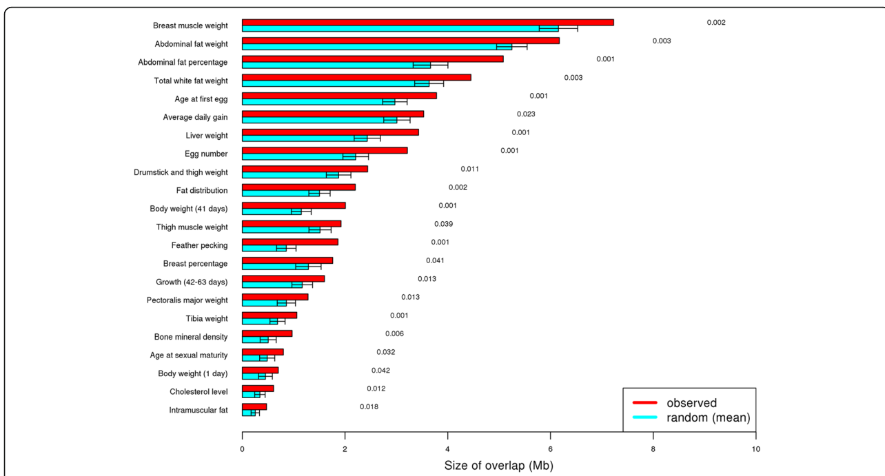
Fig. 6 Significant overlap of putative selection signature regions from SNP-based analysis with relevant chicken QTL-traits. Red bars indicate the observed overlap (selection signature regions overlapping with the respective trait), blue bars indicate the random overlap (1000 permutations), and the error bars indicate the standard deviation. The permutation p -values are listed on the right
