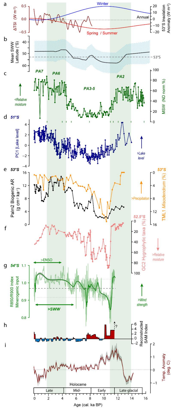
Figure 7. Regional palaeoclimate records. a) Total Solar Irradiance ( \Delta TSI) anomaly from present day value (Steinhilber et al., 2009) compared with solar insolation received at 53°S during the Holocene (Laskar et al.,
